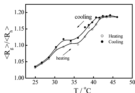
Figure 8. Temperature dependence of ratio of average radius of gyration ( \langle R_g \rangle ) to average hydrodynamic radius ( \langle R_h \rangle ) of multiblock copolymer chains in water during heating and cooling, where all the symbols and labels have the same meanings as in Figure 5. The concentration was 1.0 \times 10^{-6} g/mL, and the relative error is no more than 5% for each data point.
