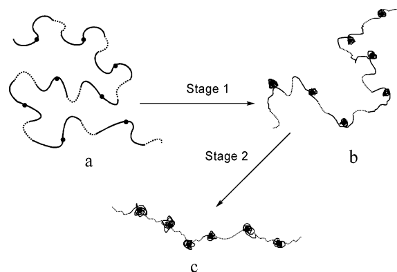
Figure 9. Schematic of the two transition stages of the multiblock copolymer chain in water during heating. The solid lines represent PNIPAM blocks, the broken lines represent PEO blocks, and the black dots represent S–S bonds.
