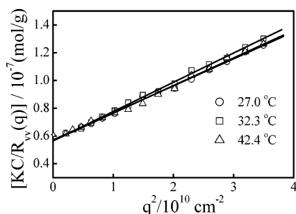
Figure 4. Scattering vector ( q ) dependence of Raleigh ratio R_{vv}(q) of multiblock copolymer chains in water, where the multiblock copolymer concentration was 1.0 \times 10^{-6} g/mL, and the relative error is no more than 5% for each data point.
