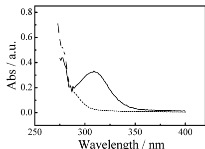
Figure 3. UV spectra of \text{C}_{12}\text{H}_{25}\text{SC}(=\text{S})\text{S-PNIPAM}_{62}\text{-}b\text{-PEO}_{23}\text{-}b\text{-PNIPAM}_{62}\text{-SC}(=\text{S})\text{S-C}_{12}\text{H}_{25} (solid line) and \text{NC}(\text{Me}_2)\text{C-PNIPAM}_{62}\text{-}b\text{-PEO}_{23}\text{-}b\text{-PNIPAM}_{62}\text{-C}(\text{Me}_2)\text{CN} (broken line) in tetrahydrofuran.
