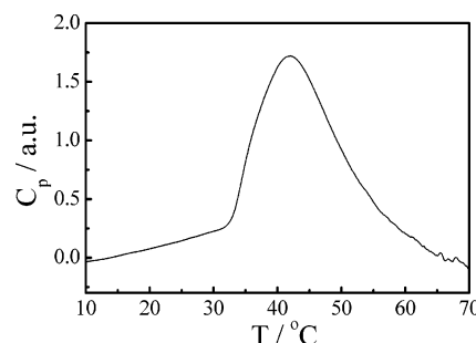
Figure 11. Temperature dependence of partial heat capacity ( C_p ) of triblock copolymer chains NC(Me 2 )C–PNIPAM 62 -b-PEO 23 -b-PNIPAM 62 -C(Me 2 )CN in water where the heating rate was 1.0 °C/min and the concentration was 1.0 \times 10^{-3} g/mL.
