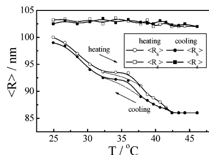
Figure 7. Temperature dependence of z-average of root-mean-square radius of gyration ( \langle R_g \rangle ) and hydrodynamic radius ( \langle R_h \rangle ) of multiblock copolymer chains in water during heating and cooling, where all the symbols and labels have the same meanings as in Figure 5. The concentration was 1.0 \times 10^{-6} g/mL, and the relative error is no more than 2% for each data point.
